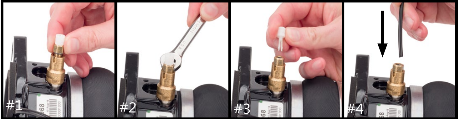
#2 拧紧接头，扭矩约为2NM (18 IN-LBS/1.5 FT-LBS)
