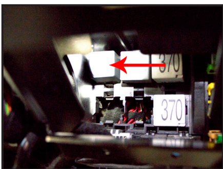
02-09 Audi A8 (w/Gas Engine) Relay located on the left side of the vehicle under the dashboard.
